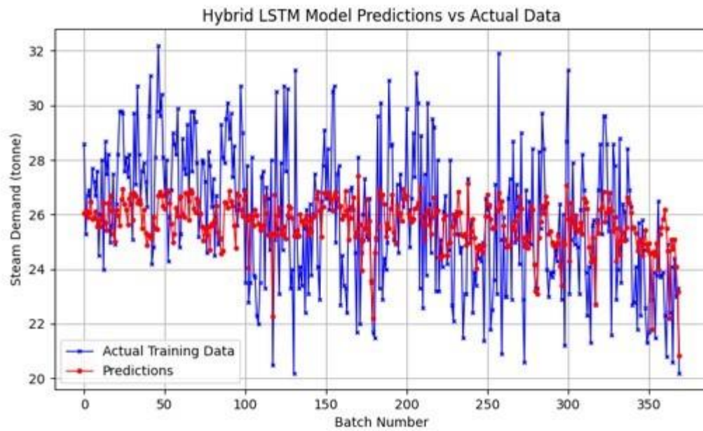
Figure SI-5: Hybrid LSTM Model Prediction on Training Data (RMSE = 2.34; MAE = 1.90)
