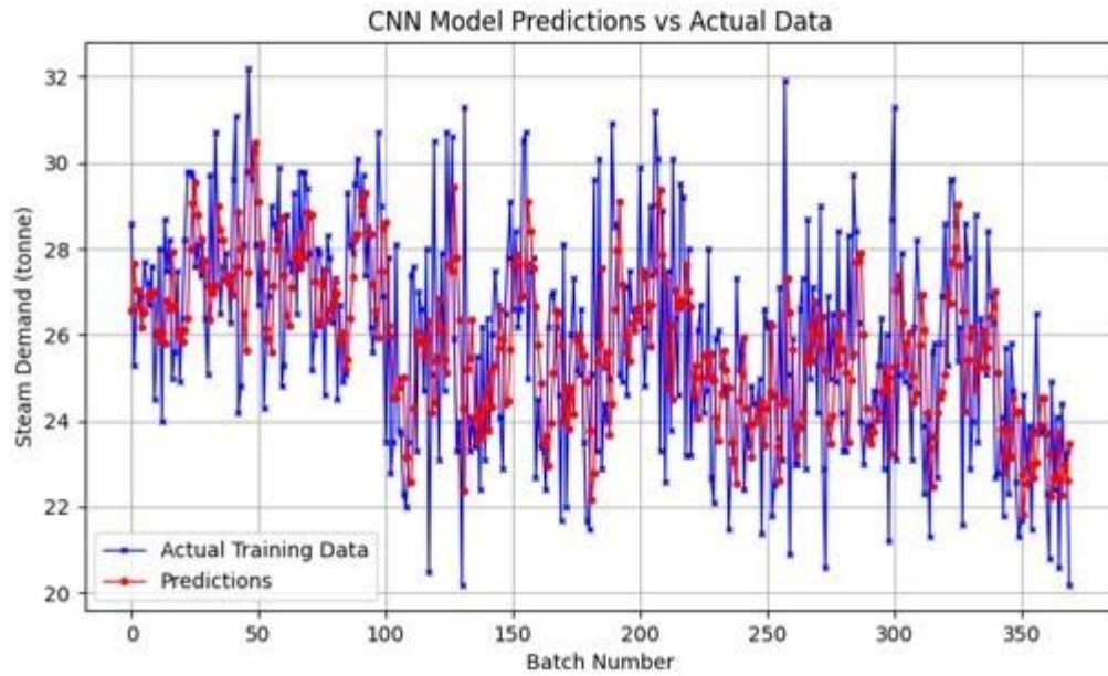
Figure SI-3: CNN Model Prediction on Training Data (RMSE = 2.50; MAE = 2.00)
