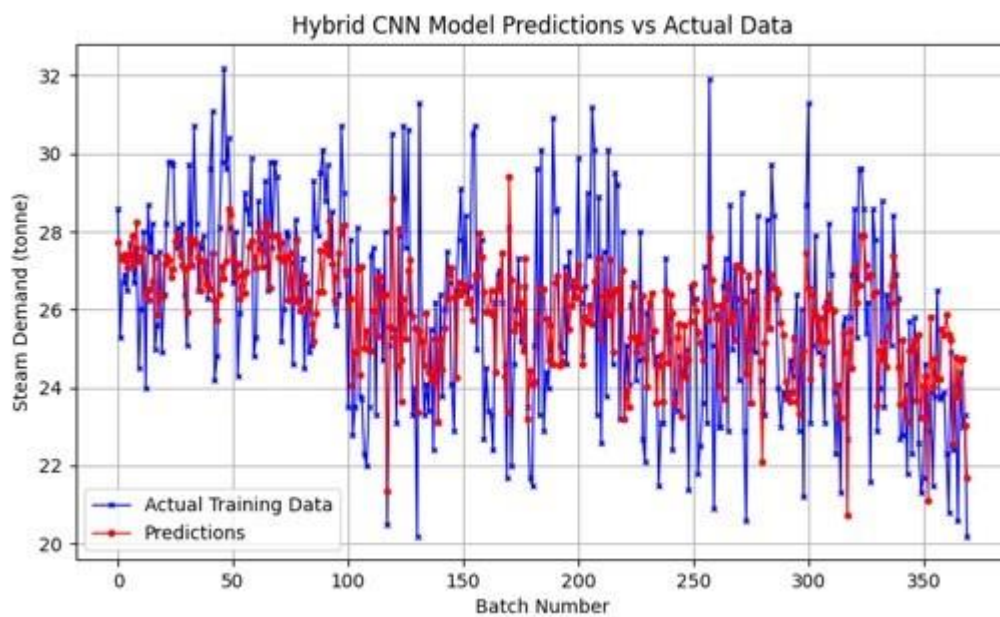
Figure SI-6: Hybrid CNN Model Prediction on Training Data (RMSE = 1.97; MAE = 1.56)
