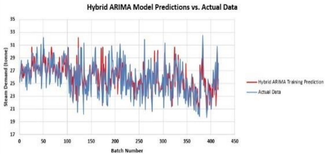
Figure SI-4: Hybrid ARIMA Model Prediction on Training Data (RMSE = 1.57; MAE = 1.26)
