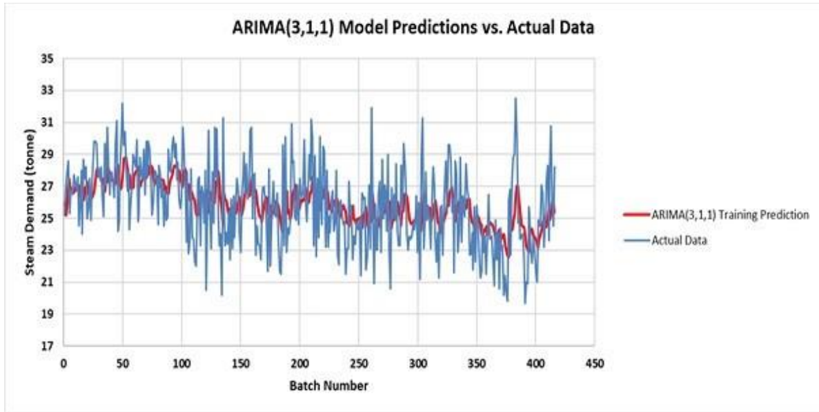
Figure SI-1: ARIMA Model Prediction on Training Data (RMSE = 2.34; MAE = 1.91)
