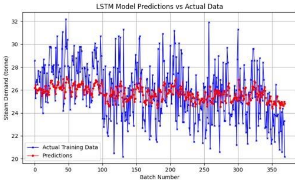
Figure SI-2: LSTM Model Prediction on Training Data (RMSE = 2.39; MAE = 1.98)
