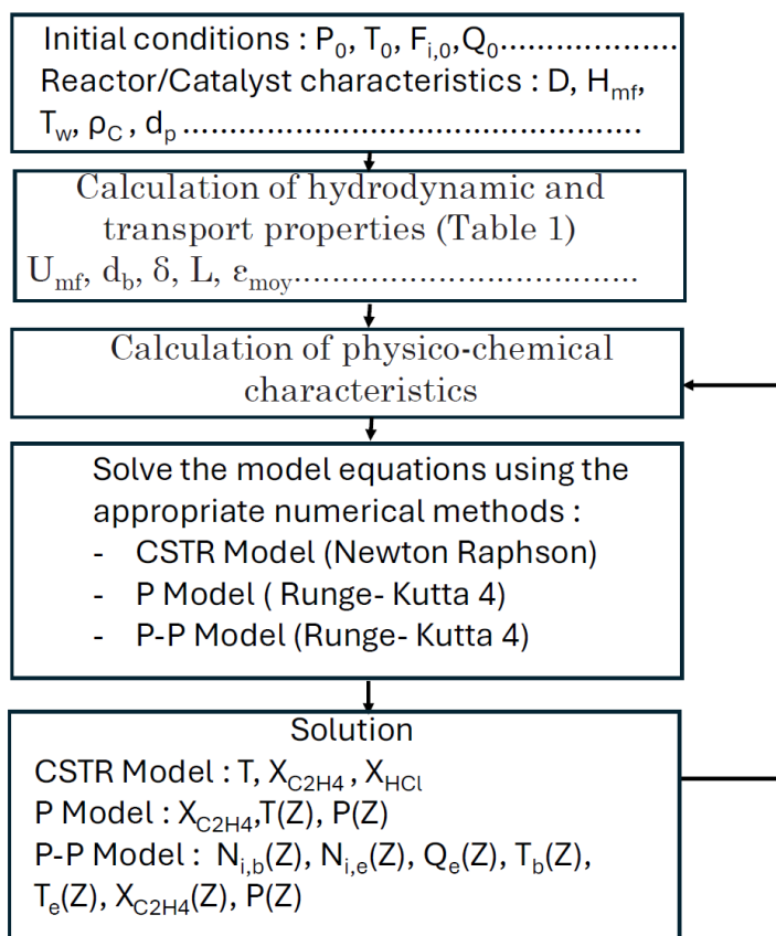
Figure S1. New Modeling Approaches for Ethylene Oxychlorination in Fluidized Bed Reactors: Industrial and Low Flow Rate Conditions.
