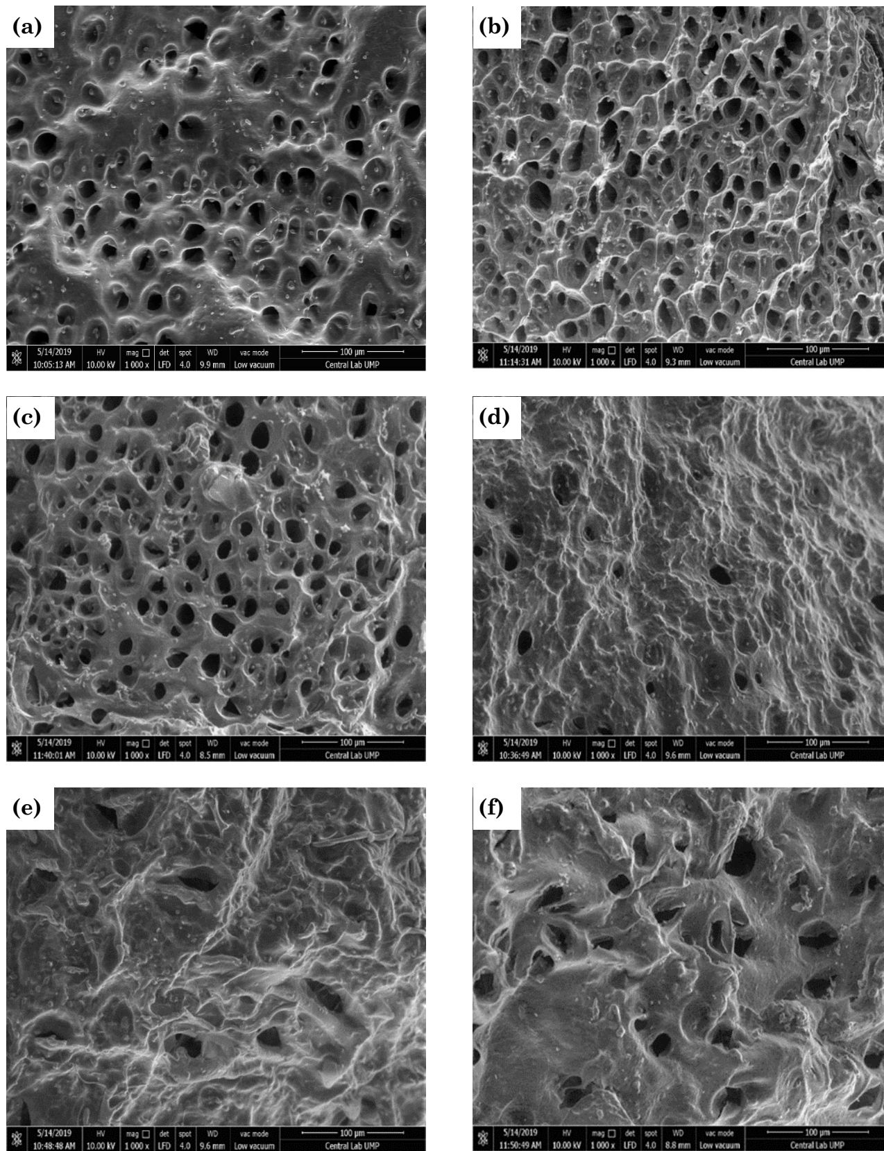
Figure 4. SEM images of a pore immobilised microalgae beads using matrix systems of (a) SA, (b) SA+GT, (c) SA+CA, (d) SA+CMC, (e) SA+CR and (f) SA+CT with 1000× magnification.
