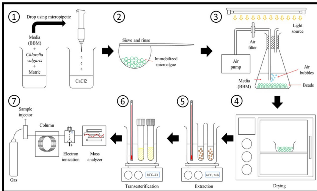
Figure 1. Schematic diagram of the main experimental setup of biodiesel production consisted of (1) preparation of the beads, (2) Sieve and rinse the beads, (3) Immobilisation culture of Chlorella vulgaris , (4) Drying the microalgae biomass, (5) Extraction process, (6) Transesterification process, (7) Analysis of fatty acid methyl ester (FAME).
