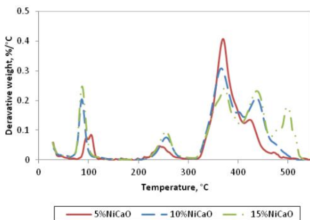
Figure 5. TGA analysis of Ni/CaO catalyst at 10 K min -1
