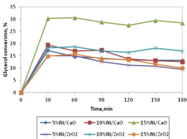
Figure 9. Glycerol conversion as function of time at 700 °C
