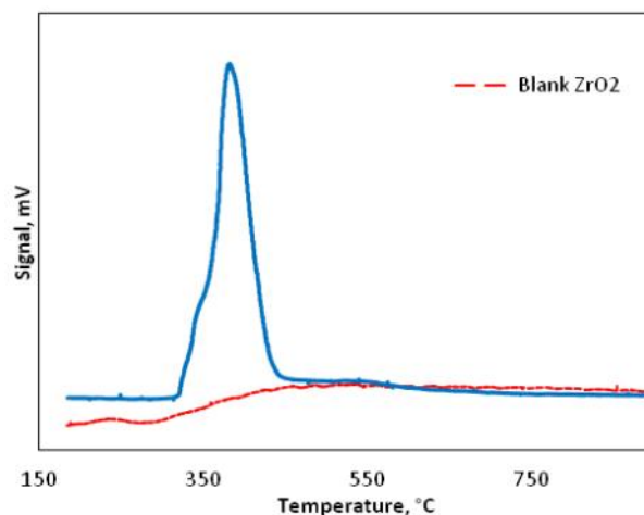
Figure 8. Temperature programmed reduction for blank ZrO 2 and 15% Ni/ZrO 2
