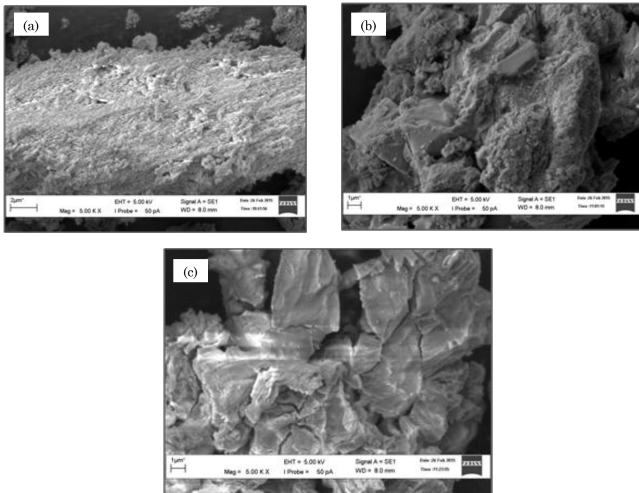
Figure 3. Morphology structure of the calcined: (a) 5% Ni/CaO, (b) 10% Ni/CaO, (c) 15% Ni/CaO was taken at magnification of 5000 times
