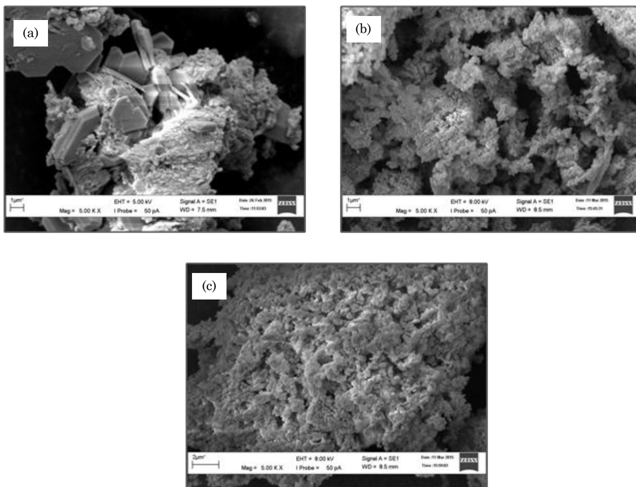
Figure 4. Morphology structure of the calcined: (a) 5% Ni/ZrO 2 , (b) 10% Ni/ZrO 2 , (c) 15% Ni/ZrO 2 was taken at magnification of 5000 times
