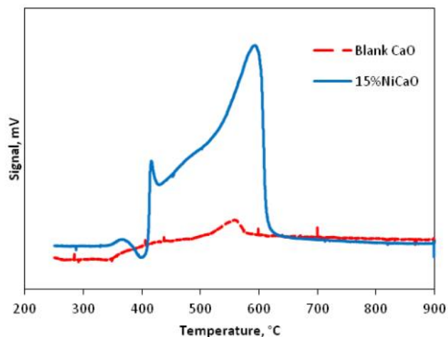
Figure 7. Temperature programmed reduction for blank CaO and 15% Ni/CaO
