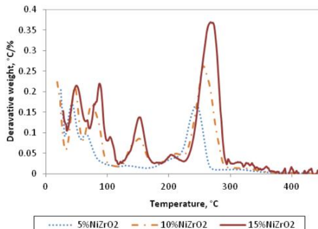
Figure 6. TGA analysis of Ni/ZrO 2 catalyst at 10 K min -1
