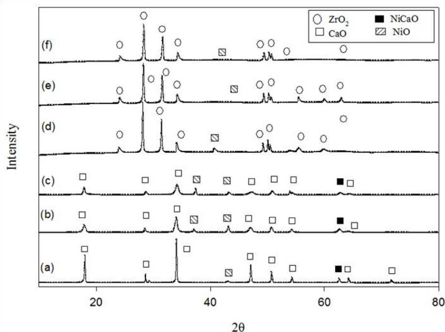
Figure 2. XRD pattern of prepared catalysts with various CaO and ZrO 2 loadings (a) 5% Ni/CaO, (b) 10%Ni/CaO, (c) 15% Ni/CaO, (d) 5% Ni/ZrO 2 , (e) 10% Ni/ZrO 2 , and (f) 15% Ni/ZrO 2
