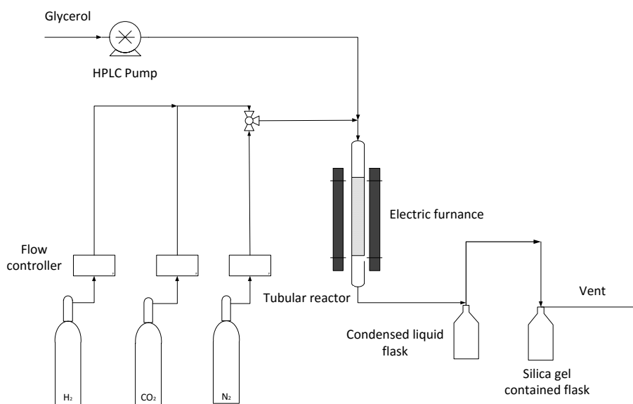
Figure 1. Experimental setup for the glycerol dry reforming
