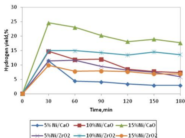
Figure 10. Hydrogen yield of Ni/CaO and Ni/ZrO 2 versus time at 700 °C
