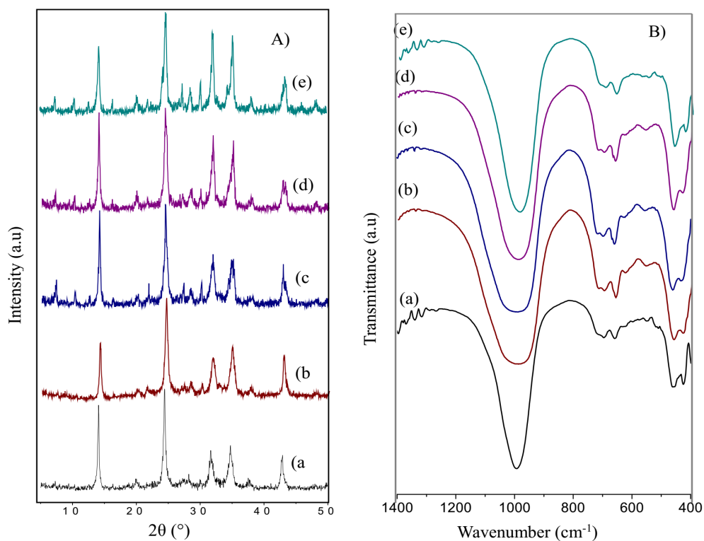
Figure 4. (A) XRD pattern, (B) FT-IR spectra for sodalite with SiO 2 /Al 2 O 3 molar ratio variations of (a) 1.5, (b) 2, (c) 2.5, (d) 3, (e) 3.5
