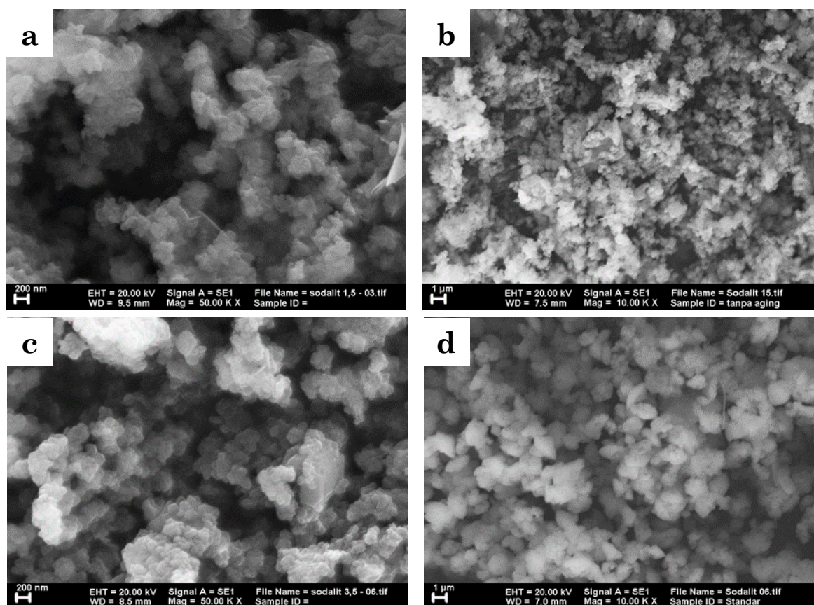
Figure 5. The morphology of synthesis results based on SEM characterization on the SiO 2 /Al 2 O 3 molar ratio variations of (a) 1.5, (b) 2, (c) 3.5, and (d) standard sodalite
