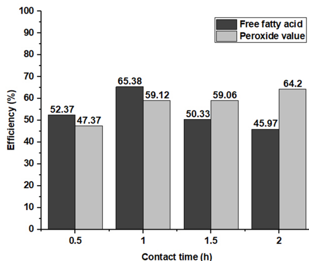
Figure 9. Optimization of the UCO photodegradation reaction time.
