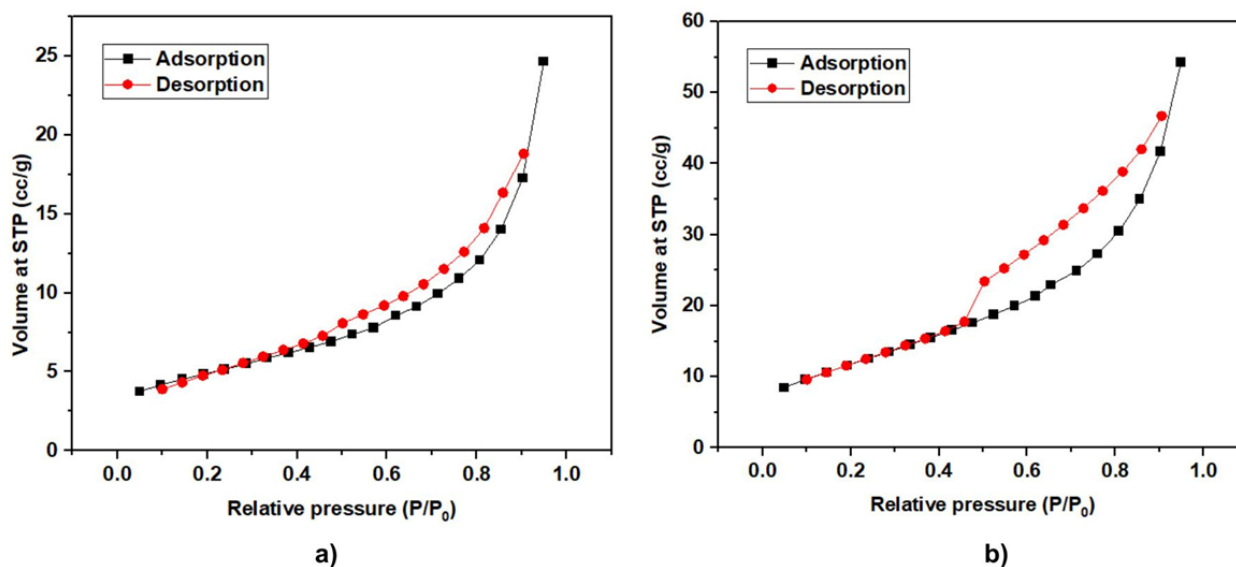
Figure 3. Adsorption-desorption isotherm curve of TiO_2/ZnO/CuO composites, a) 0 CMC and b) 1 CMC.
