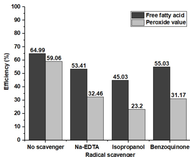
Figure 12. UCO photodegradation performance on various radical scavengers.
