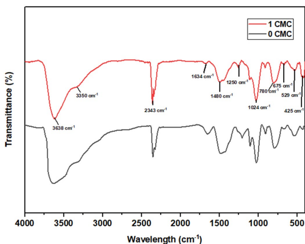
Figure 1. FTIR spectrum of \text{TiO}_2/\text{ZnO}/\text{CuO} 0 CMC and 1 CMC composites.
