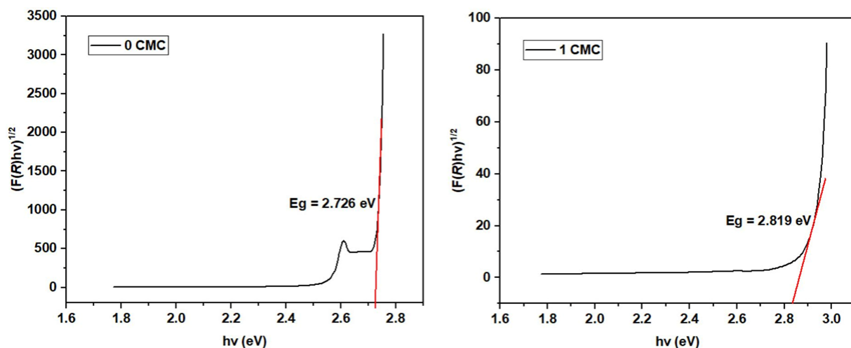
Figure 5. Tauc plot of indirect TiO 2 /ZnO/CuO 0 and 1 CMC composites.
