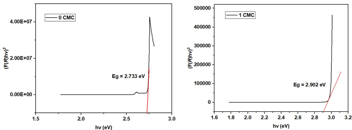
Figure 6. Tauc plot of direct TiO 2 /ZnO/CuO 0 and 1 CMC composites.
