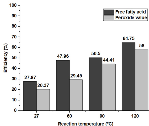
Figure 10. Optimization of the UCO photodegradation reaction temperature.
