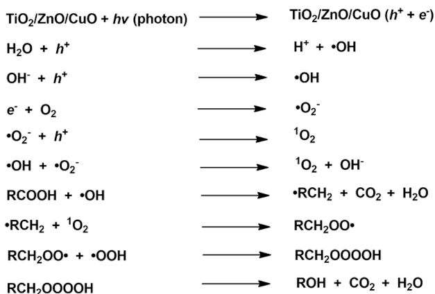
Figure 14. Mechanism of radical photodegradation of UCO.
