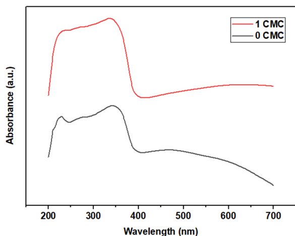
Figure 4. UV-Vis absorbance of TiO_2/ZnO/CuO 0 and 1 CMC composites.
