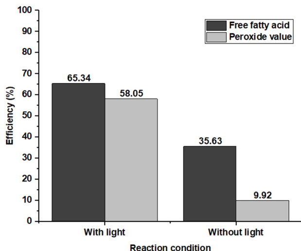
Figure 8. Photocatalyst performance under dark and light conditions.
