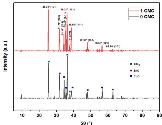
Figure 2. XRD spectrum of \text{TiO}_2/\text{ZnO}/\text{CuO} 0 CMC and 1 CMC composites.
