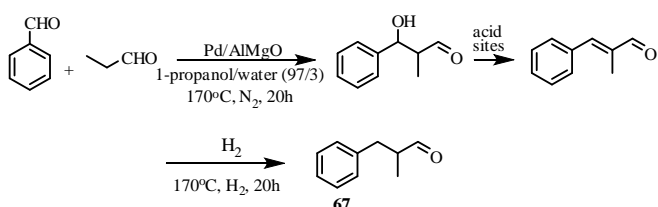
Scheme 40. One-pot synthesis of 2-methyl-3-phenyl-propenal
