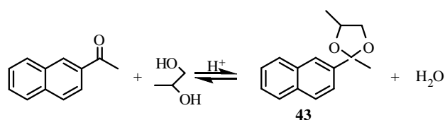
Scheme 21. Reaction scheme of the formation of 2-methyl-2-naphthyl-4-methyl-1,3-dioxolane ( 43 )
