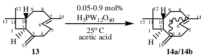
Scheme 6. Acetoxylation of \beta -caryophyllene
