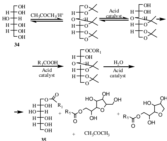
Scheme 13. One-pot synthesis of sorbitol fatty acid esters
