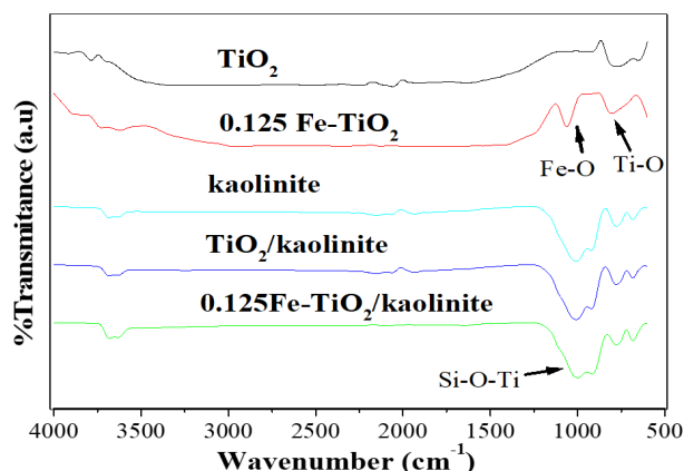
Figure 2. FTIR Spectra pattern for TiO 2 /kaolinite and Fe-doped TiO 2 /kaolinite.
